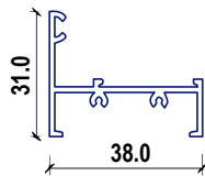
ALN 174 JAMBA
