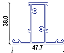
ALN 292 DIVISOR
