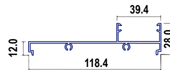
ALN 708 JAMBA 8025
